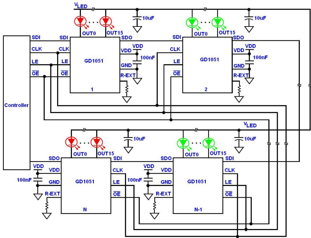
Serial connection of GD1051
