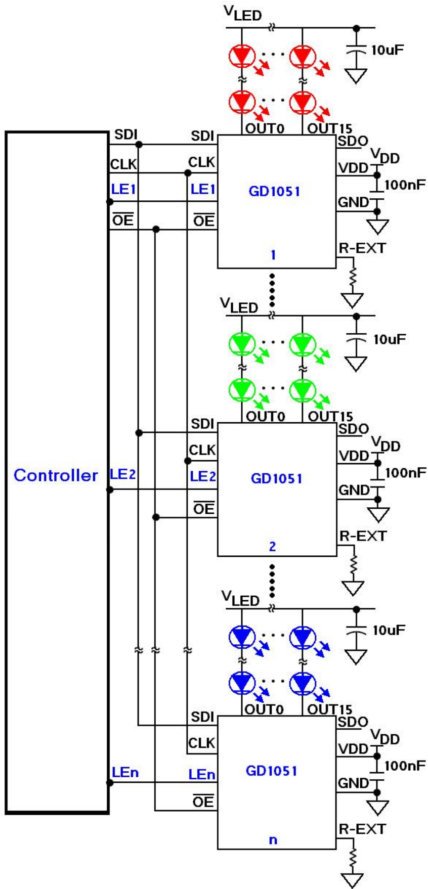
Parallel Connection of GD1051
